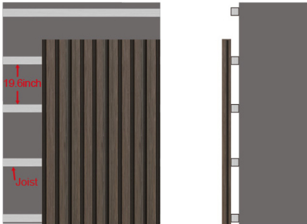
Vertical Installation
