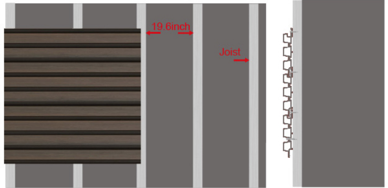
Horizontal Installation
