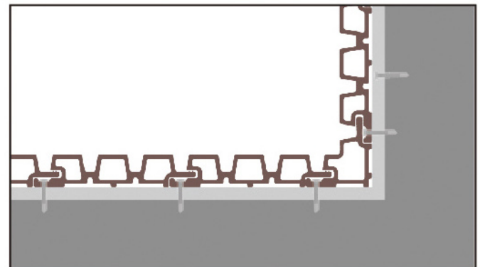
Inside Corner-Option 2
