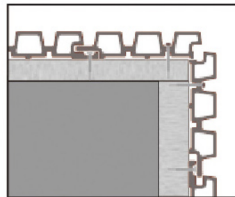
Outside Corner-Option 2
